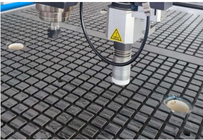
Vacuum Adsorption Table
